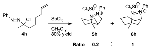
Scheme 2. Preferential Formation of Bridged Bicyclic 7-Membered-Ring-Containing Diazenium Salt
