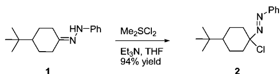
Scheme 1. Sulfonium Salt Mediated \alpha -Chloroazo Formation
