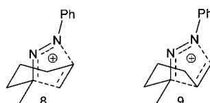
Figure 1. Possible transition states leading to the formation of diazenium salts 5e and 6e .
